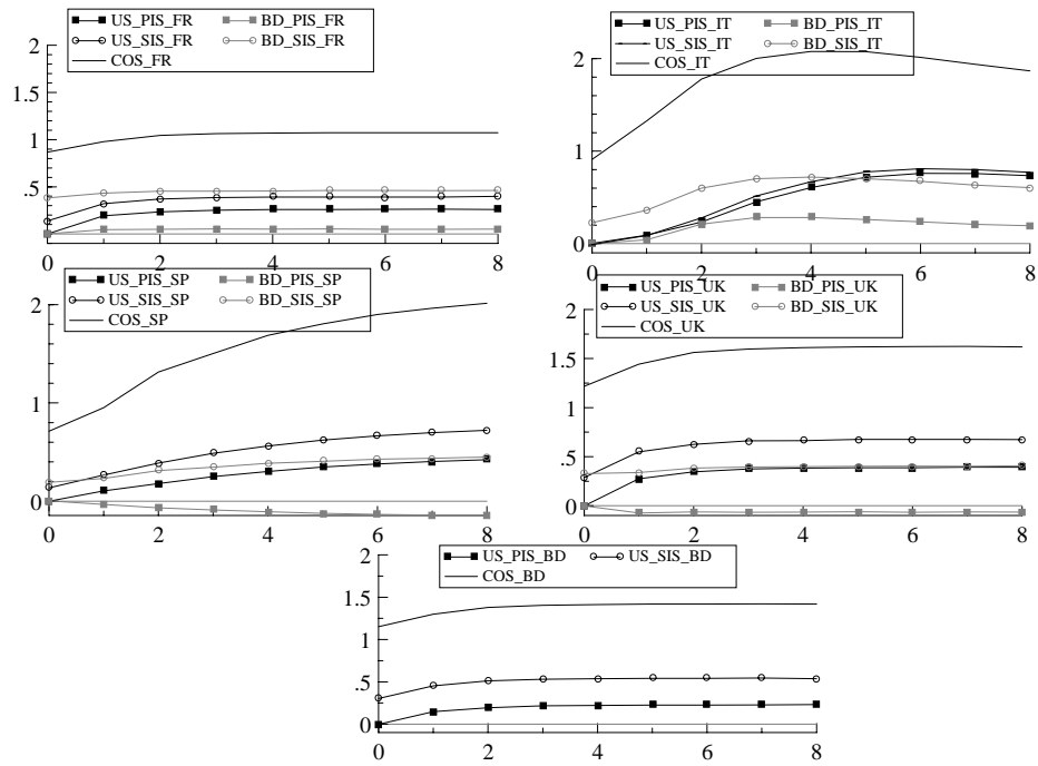
Figure 1 Accumulated Generalized Responses for France, Italy, Spain, UK and Germany to PIS and SIS shocks from US and Germany (BD) and to a common shock (COS) computed using trivariate VARs .
