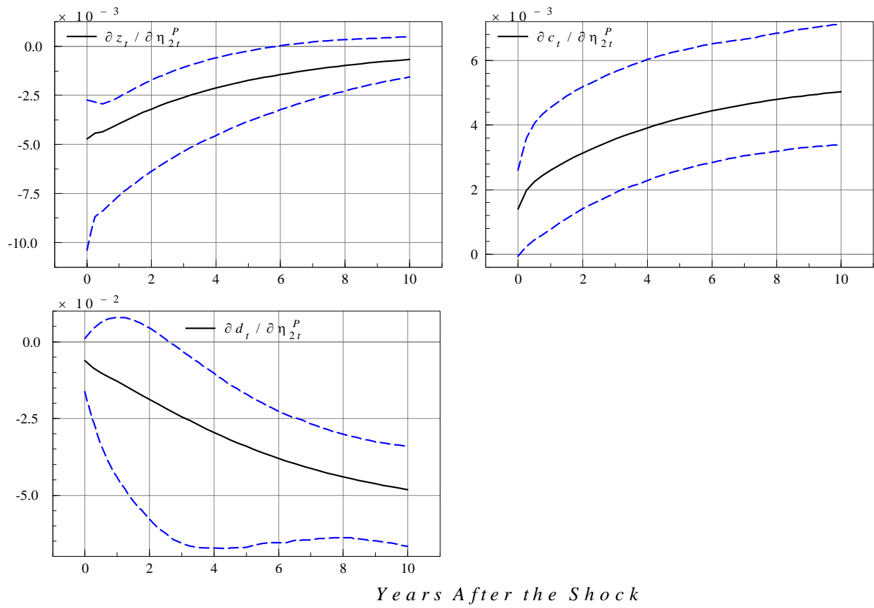
Figure 3. Impulse Responses to the Second Permanent Shock.
