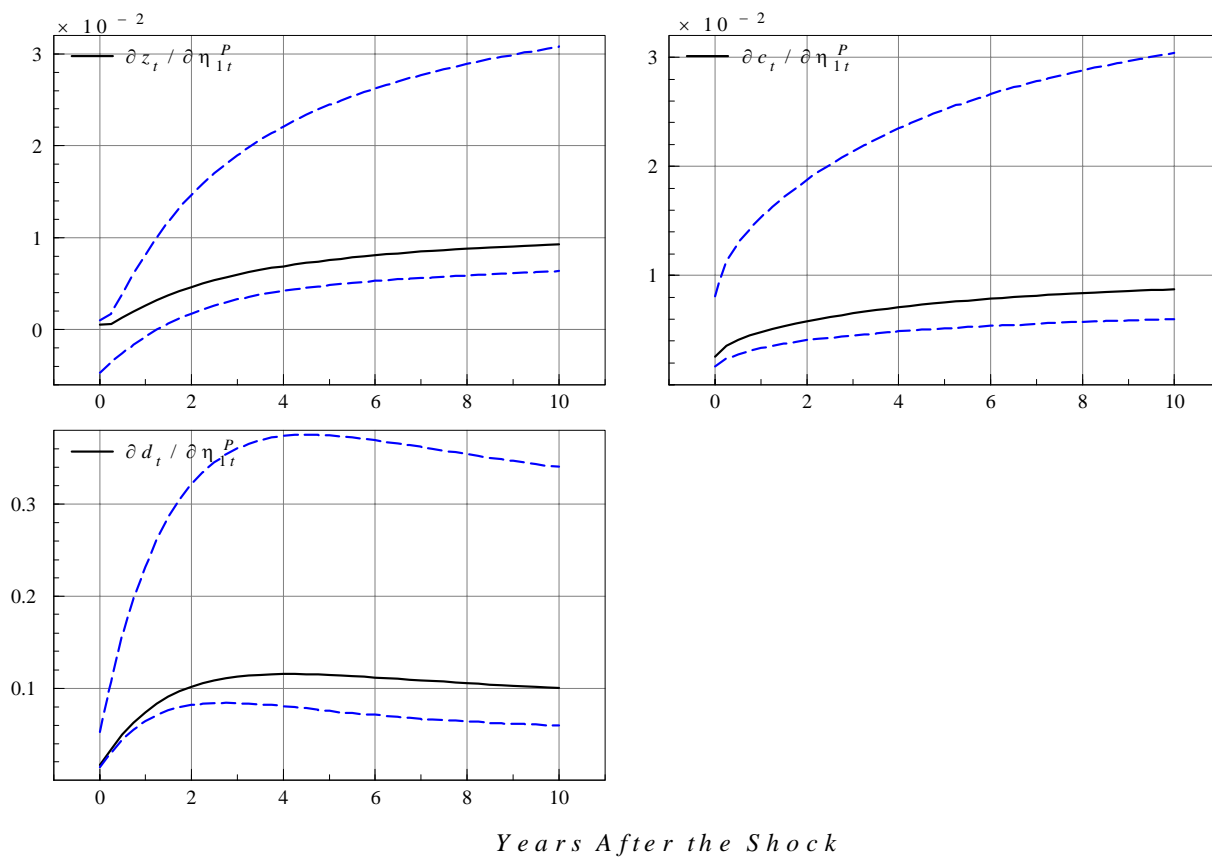
Figure 2. Impulse Responses to the First Permanent Shock.
