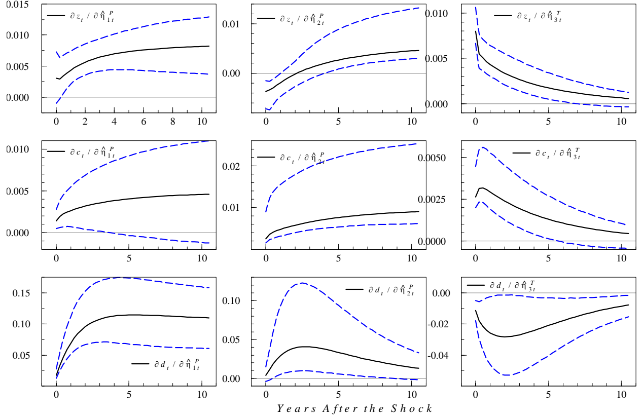
Figure 4. Alternative Identification Scheme I - Impulse Responses.
