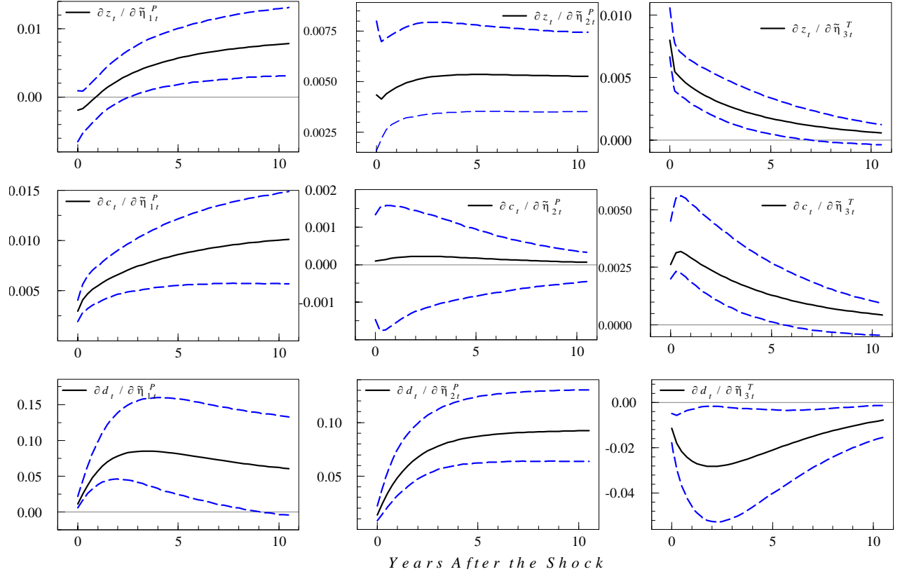
Figure 5. Alternative Identification Scheme II - Impulse Responses.
