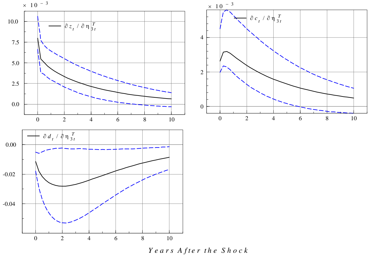
Figure 1. Impulse Responses to the Transitory Shock.
